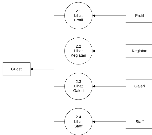
Gambar 3.4 DFD Level 2 Proses 1
