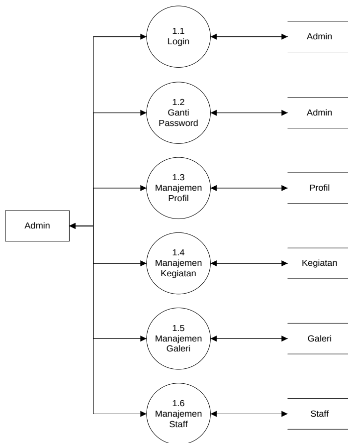
Gambar 3.3 DFD Level 2 Proses 1
